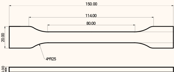
TENSILE TESTING SPECIMEN ISO 527
