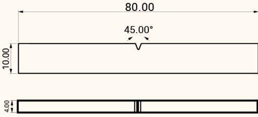
IMPACT TESTING SPECIMEN ISO 179
